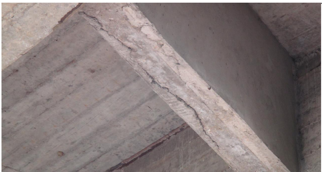
PR 47 + 750
