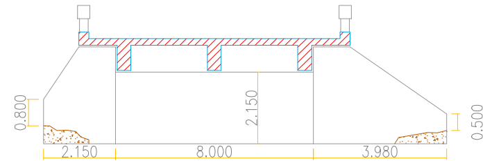
CORTE (A-A') ES1
