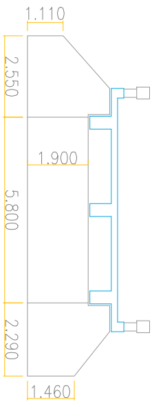
CORTE (A-A') ES1
